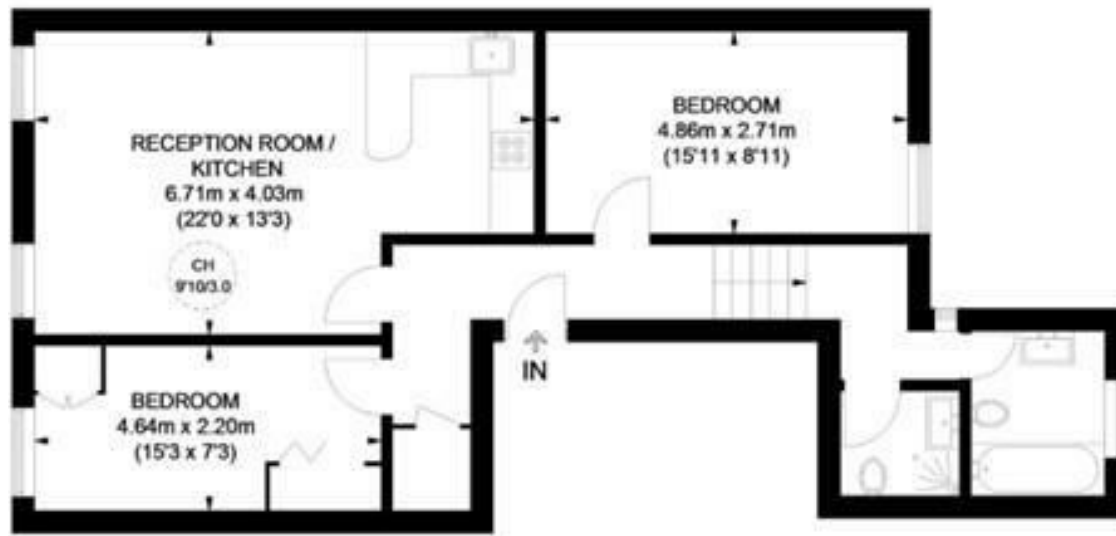
SECOND FLOOR
